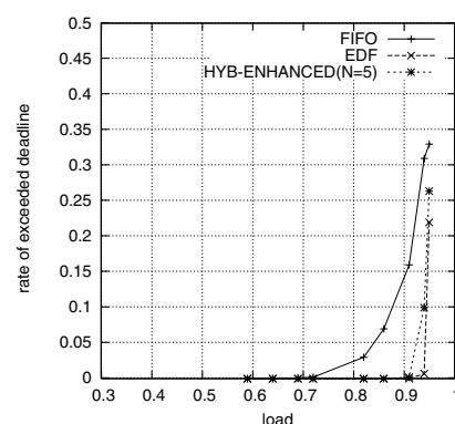
Fig. 7. Comparison EDF, FIFO and HYB-ENHANCED (N=5) "Exponentially Distributed ON/OFF Traffic", with deadline set \mathcal{D}_2 .
