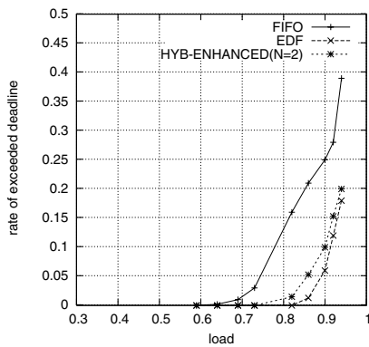
Fig. 5. Comparison EDF, FIFO and HYB-ENHANCED (N=2) "Pareto Distributed ON/OFF Traffic", with deadline set \mathcal{D}_1 .
