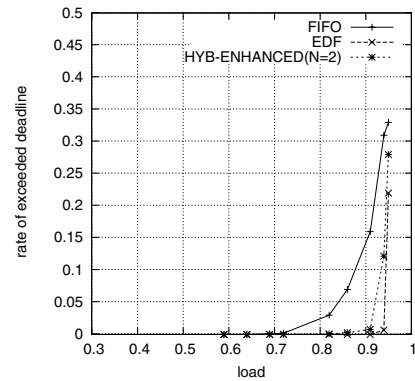
Fig. 3. Comparison EDF, FIFO and HYB-ENHANCED (N=2) "Exponentially Distributed ON/OFF Traffic", with deadline set \mathcal{D}_1 .
