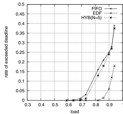
Fig. 8. Comparison EDF, FIFO and HYB (N=5) "Pareto Distributed ON/OFF Traffic", with deadline set \mathcal{D}_2 .
