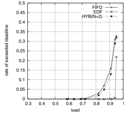
Fig. 2. Comparison EDF, FIFO and HYB (N=2) "Exponentially Distributed ON/OFF Traffic", with deadline set \mathcal{D}_1 .
