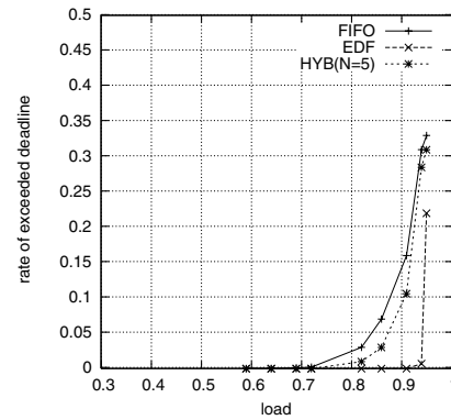
Fig. 6. Comparison EDF, FIFO and HYB (N=5) "Exponentially Distributed ON/OFF Traffic", with deadline set \mathcal{D}_2 .
