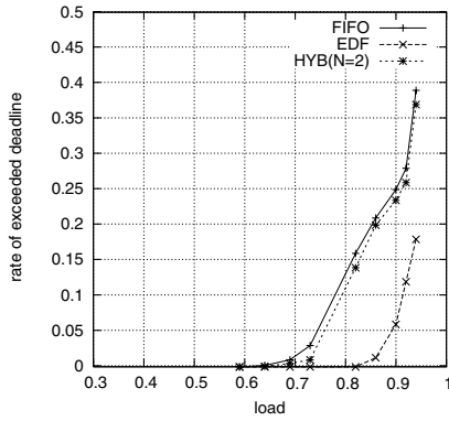
Fig. 4. Comparison EDF, FIFO and HYB (N=2) "Pareto Distributed ON/OFF Traffic", with deadline set \mathcal{D}_1 .
