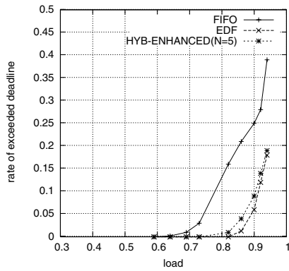
Fig. 9. Comparison EDF, FIFO et HYB-ENHANCED (N=5) "Pareto Distributed ON/OFF Traffic", , with deadline set D_2 .
