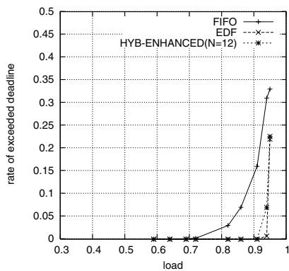
Fig. 10. Comparison EDF, FIFO and HYB-ENHANCED (N=12) "Exponentially Distributed ON/OFF Traffic", , with deadline set D_2 .
